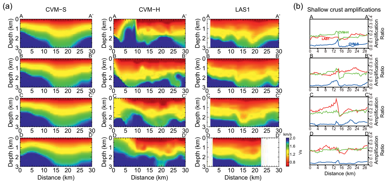
Figure 10. Comparison of our inverted LAS1 Vs model with CVM-S and CVM-H models. (a) Model comparisons for 4 cross sections in Figure 9. (b) Prediction of strong motion amplifications along the 4 cross sections using these Vs models. The red, blue and green lines indicate synthetics from the LAS1, CVM-S and CVM-H Vs models, respectively. The gapped Vs for the LAS1 cross sections are filled by replicating existing Vs at the edges to the ends of cross sections, where the amplification fluctuations are due to the reflections and scatterings in the 2D simulations.
