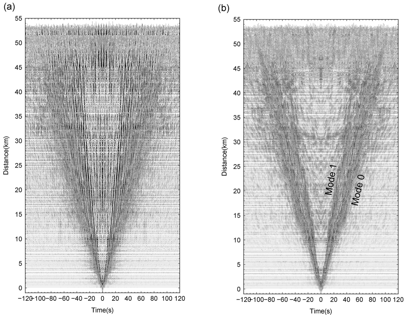
Figure 2. Inter-array noise correlation functions between SCSN stations and dense nodal arrays. (a) Noise correlation functions stacked in distance bins between 0.2 and 2.0 Hz. (b) High frequency (0.5–2.0 Hz) filtered noise correlation functions stacked in distance bins.
