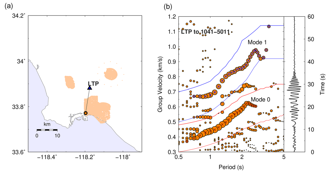
Figure 4. Example of labeling of dispersion curves. (a) The raypath from broadband station LTP (black triangle) to a dense array station 1041–5011 (orange circle). (b) The FTAN image (period axis uses a logarithmic scale) of the noise correlation function for the raypath in (a). The size of each circle is proportional to the wave packet energy at the corresponding period and group velocity. The red and blue crosses are the picked dispersion data for the fundamental mode and first overtone, respectively. The red and blue lines indicate the corridors for these two modes. The waveform to the right indicates the time-domain noise correlation function.
