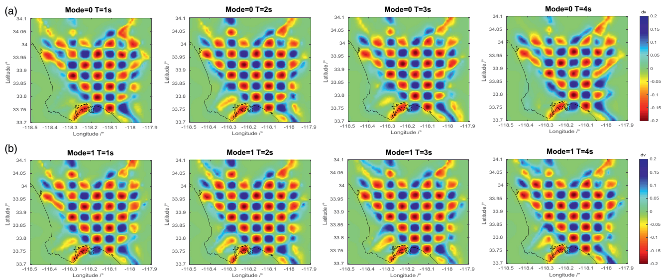
Figure 7. Checkerboard resolution maps of (a) the fundamental mode and (b) the first overtone Rayleigh wave group velocity tomography for periods 1–4 s.
