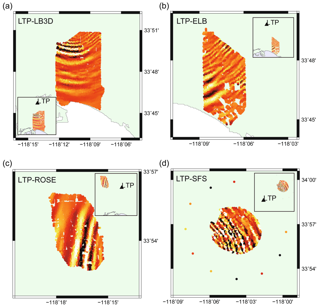
Figure 3. Wavefield snapshots of the noise correlation functions from station LTP to dense arrays (a) LB3D, (b) ELB, (c) ROSE and (d) SFS.
